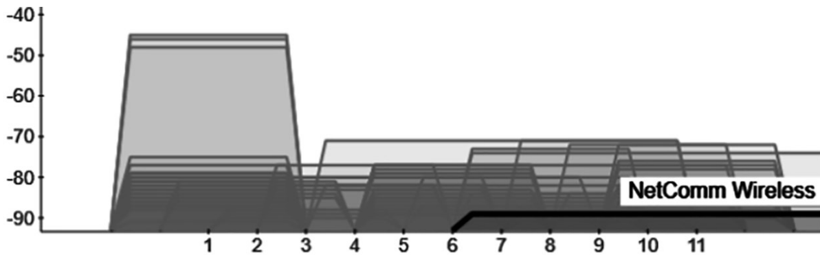
Figure 1. A typical example of, per AP, the signal strength (dBm) vs. Wi-Fi channel number in the 2.4 GHz band, as observed in a densely populated apartment block.
