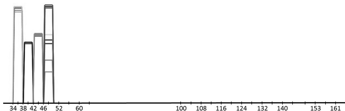
Figure 3. Relative signal strength vs. Wi-Fi channel number in the 5 GHz band, as observed in the head office of TNO in The Hague, The Netherlands.
