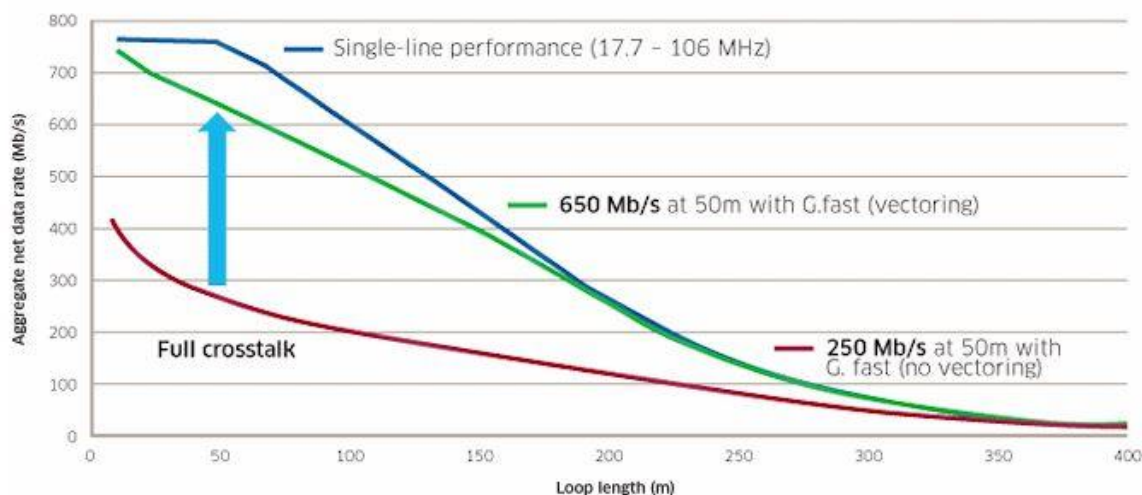
Figure 2. Data rate as a function of cable length
