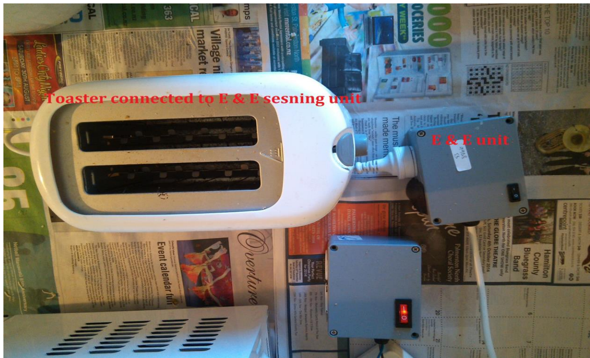
Figure 5. Toaster plugged to wellness protocol based E & E power usage and control unit
