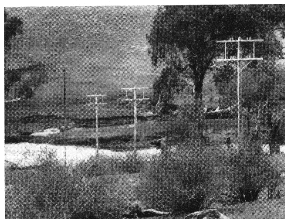
Fig. 7.—Campaspe River crossing at Axedale.
