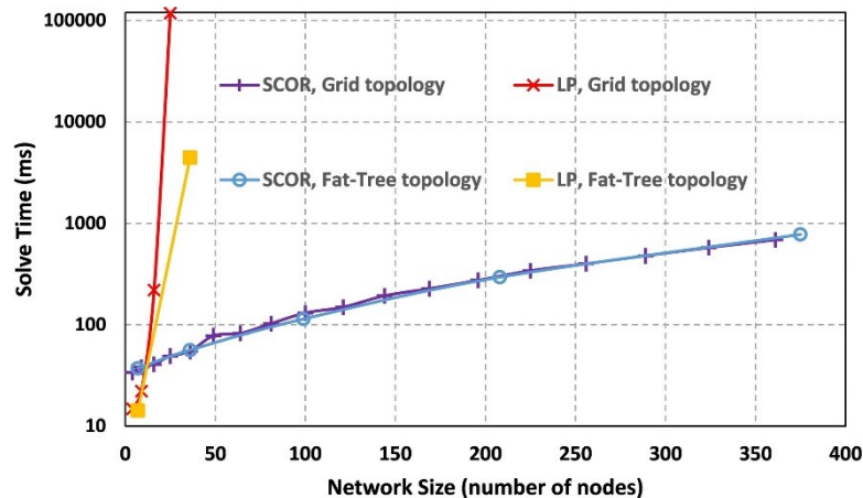
Figure 6: The solution time for the Maximum Residual Capacity problem compared to LP in fat-tree and grid topologies with various network sizes
