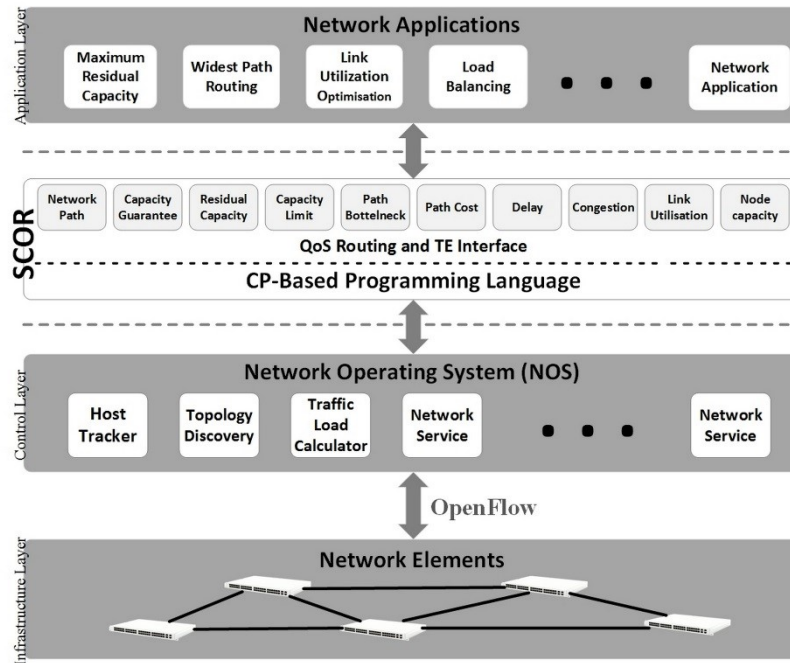
Figure 2 : Situation of SCOR in the SDN architecture
