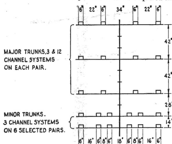
Fig. 1.—Pole Plan, showing ultimate number of pairs.
