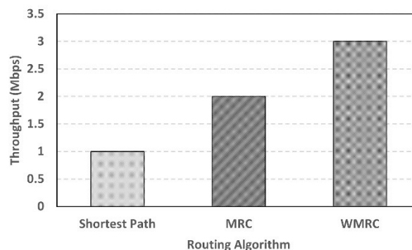
Figure 4: Theoretical throughput for three concurrent flows of 1 Mbps in a half duplex network with a topology as shown in Fig. 3 (node S_1 is the source and node S_7 is destination) in the case of Shortest path routing, MRC and WMRC models
