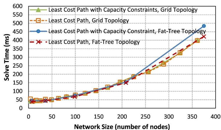
Figure 5: Solve time for the Least Cost Path and Least Cost Path with Capacity Constraint problem in fat-tree and grid topologies with various network sizes
