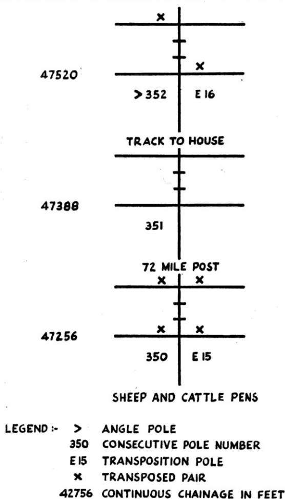
Fig. 8.—Field Book—typical sheet.
