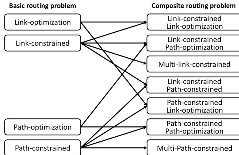
Figure 1 : Basic and composite QoS routing problems (Chen & Nahrstedt 1998)
