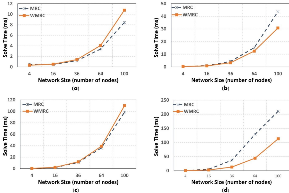
Figure 7: The solution time for the Maximum Residual Capacity (MRC) model and Wireless Maximum Residual Capacity (WMRC) model in grid topologies with various network sizes in the case a) One flow, b) Two concurrent flows, c) Three concurrent flows, and d) Four concurrent flows
