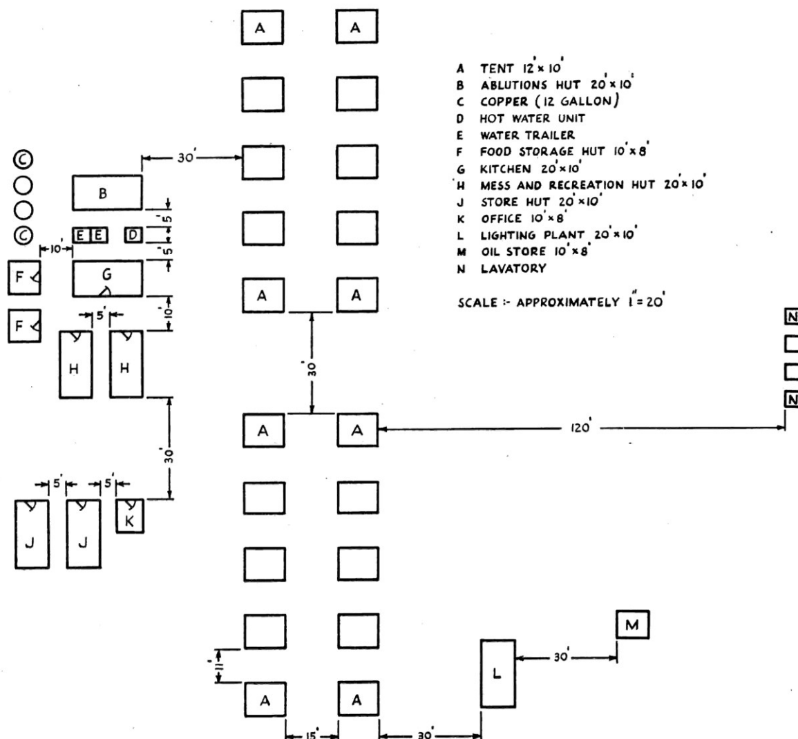
Fig. 9.—Large Line Camp—Layout.
