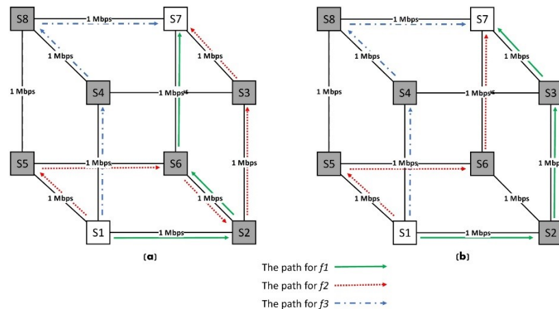
Figure 3: Paths found for three concurrent flows from node 1 to node 7 using a) Maximum residual capacity model (MRC), and b) Wireless maximum residual capacity model (WMRC)
